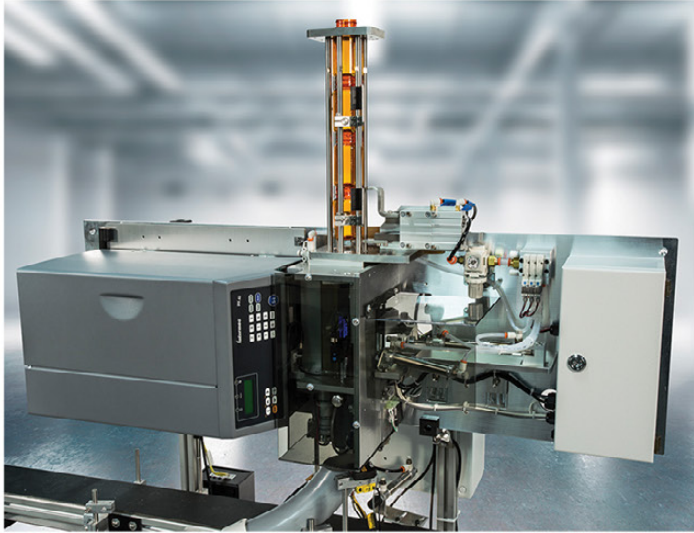
Labels 900 Bottles Per Hr Speeds of 4" to 8" Per Sec
